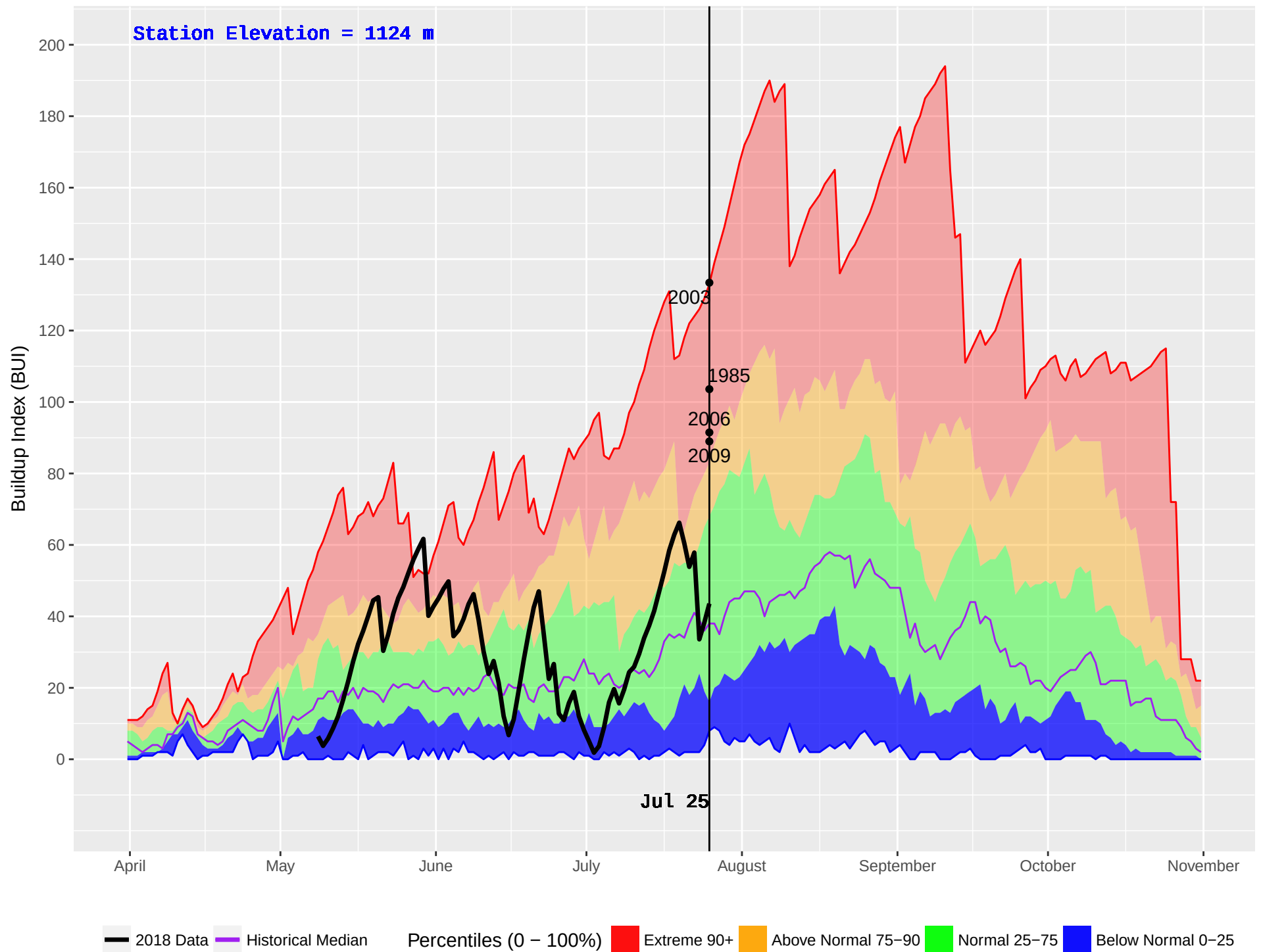
COLDSCAUR LAKE (232) : Historical (1979–2016) and Current (2018) Noon Buildup Index (BUI)
